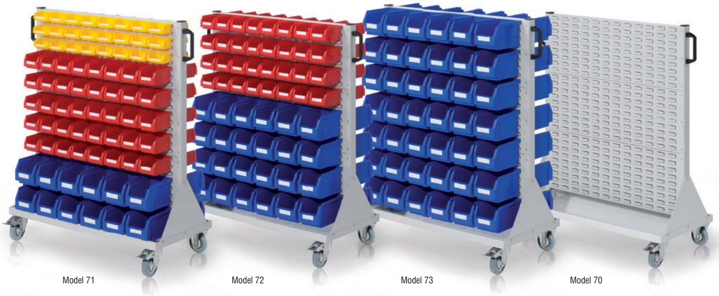
RasterMobil® Trolleys - Size 3 H 1230 x W 1000 x D 500 mm - double sided
